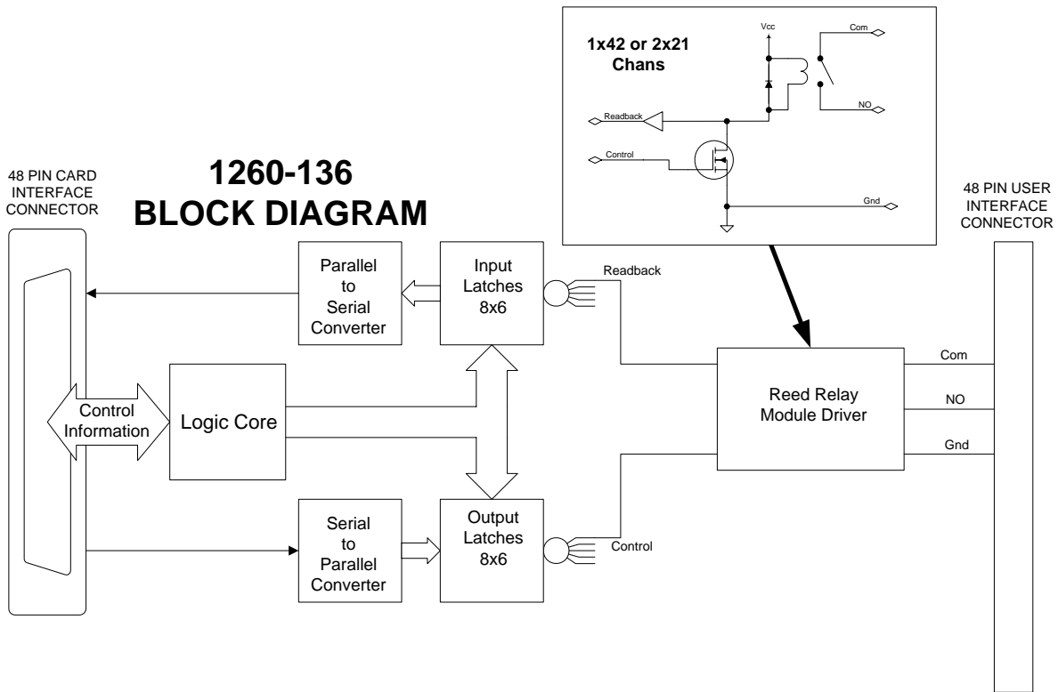
Figure 2-3, Block Diagram
